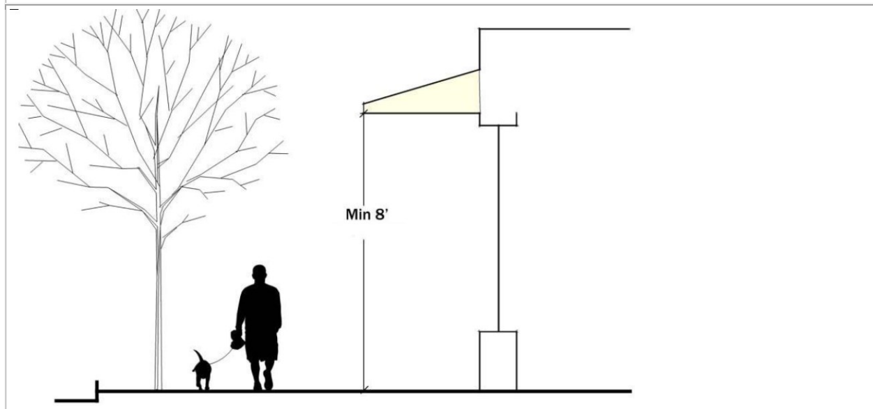
FIGURE 536-7 WEATHER PROTECTION
