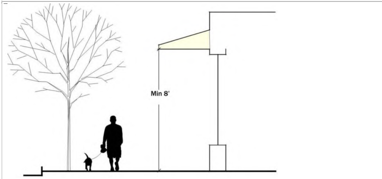
FIGURE 536-7 WEATHER PROTECTION
