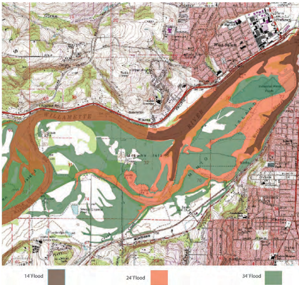
Figure 30. Flood patterns.
