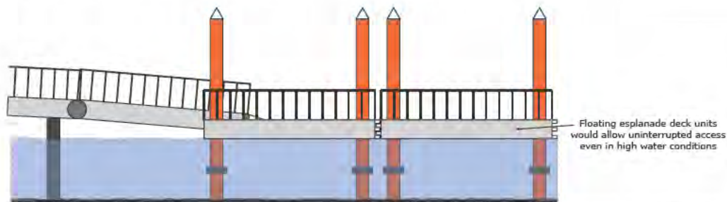
Figure 41. Esplanade cross-section.
