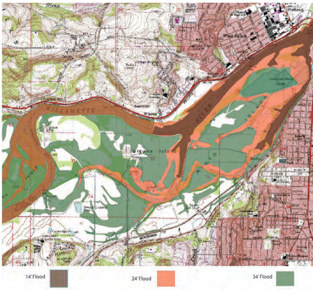
Figure 9. Flood patterns.
